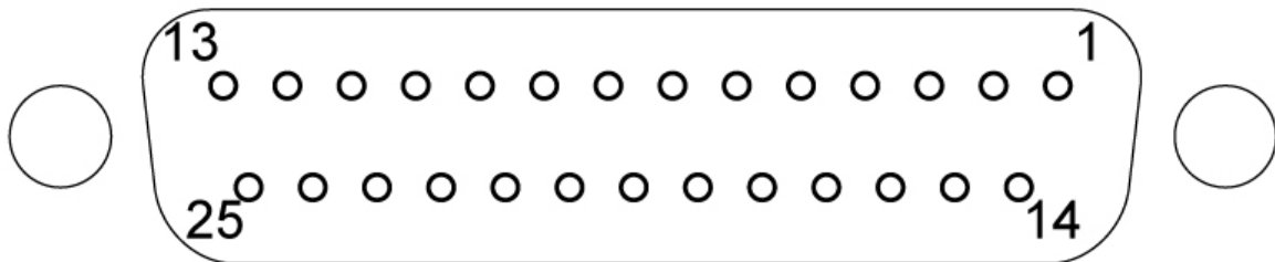
25 Way Female Sub D Connector
